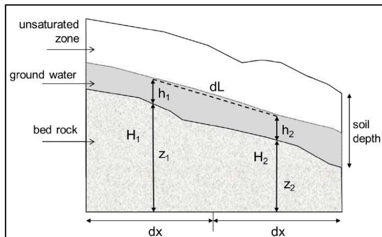
Figure 5.26: Principles of groundwater flow used in our PCRaster model: h_1 and h_2 are groundwater levels, z_1 and z_2 absolute elevation above a given datum, dL is the distance between two points along the water surface. [74]
