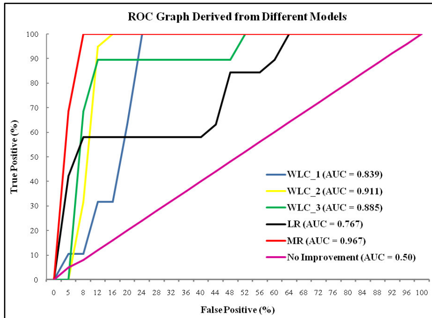
Figure 5.18: Assessment of the model performance based on the ROC curves.
