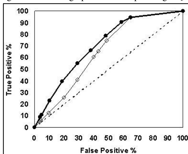
Figure 5.17: ROC graph for three input images. [60]
