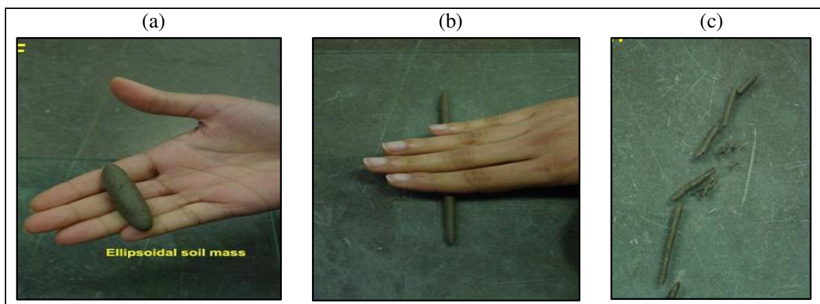
Figure 4.12: Determination of plastic limit.
