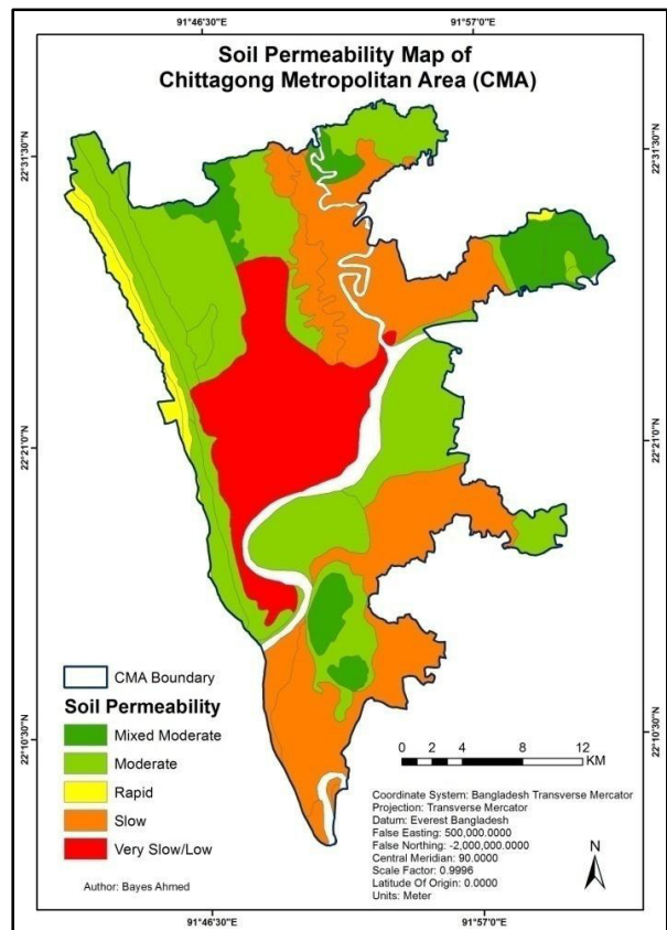
Figure 5.11: Soil permeability map.
