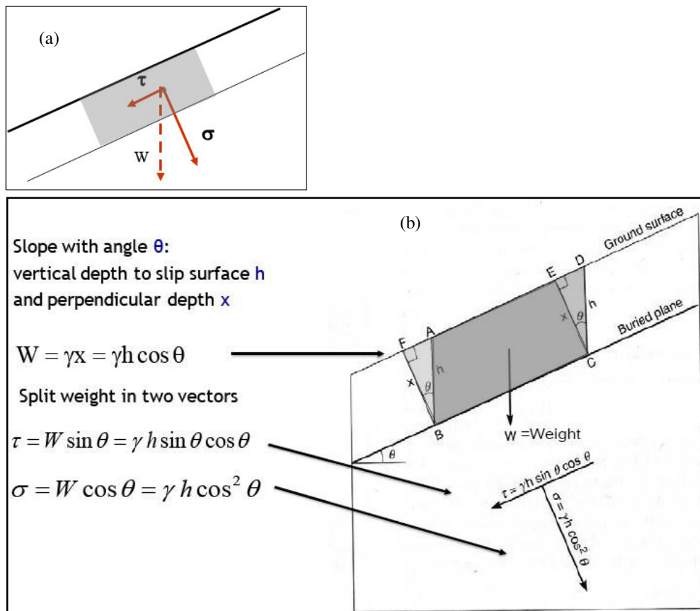
Figure 5.27: (a) weight W of a slope segment divided in a normal stress vector \sigma and shear stress vector \tau . (b) Definition of shear stress and normal stress (N/m 2 ) on a slope with a given angle \theta and regolith depth h (m). x = the regolith depth perpendicular to the slope (m) and \gamma (gamma) is the specific weight (see table 4.1, in kN/m 3 ). [75]
