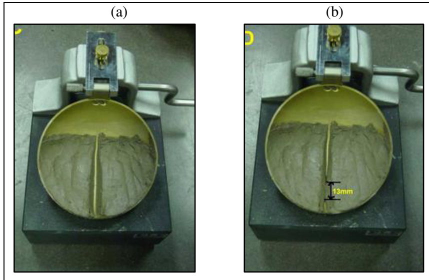
Figure 4.11: Determination of liquid limit.
