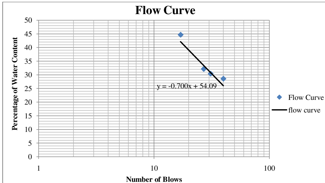
Figure 4.14: Flow curve- percentage of water content and number of blow (Moti Jharna Cluster).
